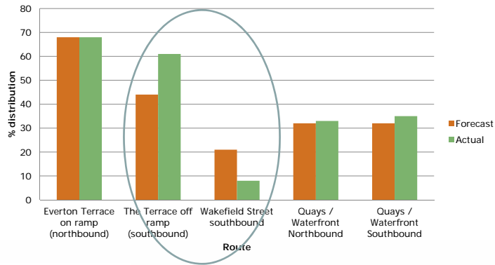
% Distribution of Terrace Tunnel traffic on key routes Forecast v Actual
