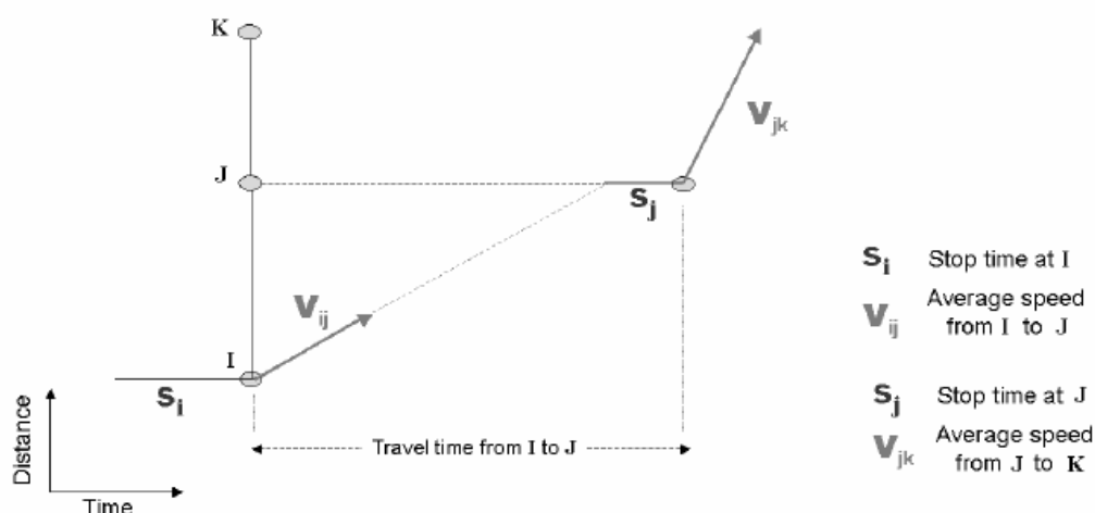
Figure 4 – Estimation of travel times between 2 consecutive SCATS signals
